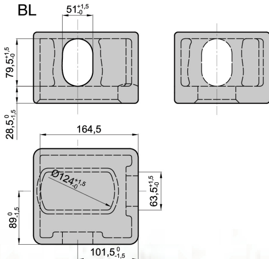
Bottom corner fitting
